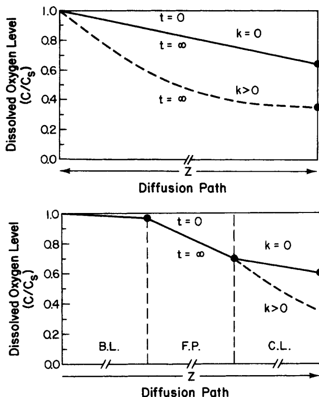
Figure 5. Concentration profiles of the one (top) and three (bottom) layer diffusion models.
